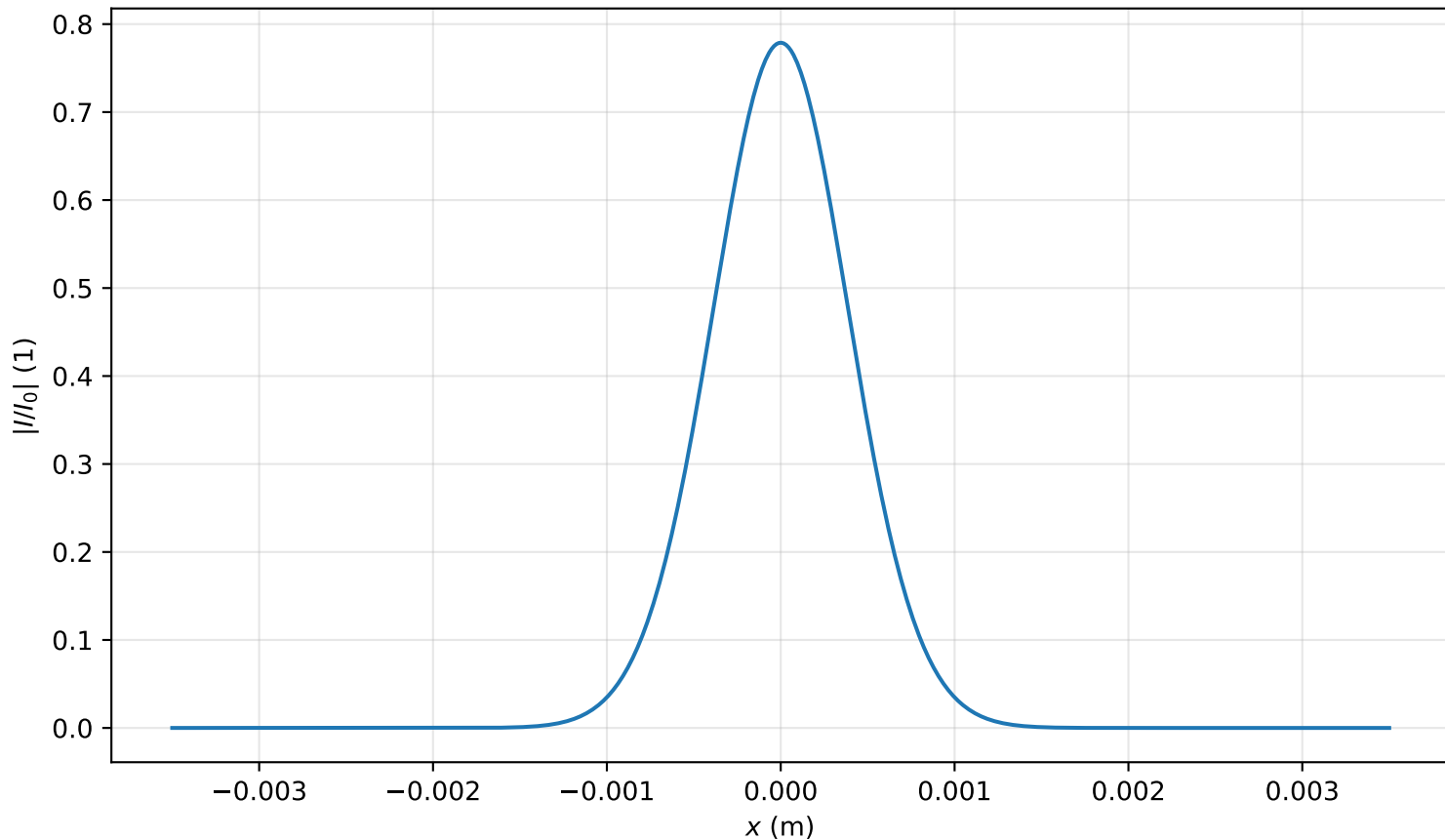
Intensity profile I(x, y = 0, z = 1.194m)/I_0 , P_{in}=0.1P_{cr} , artificial time
